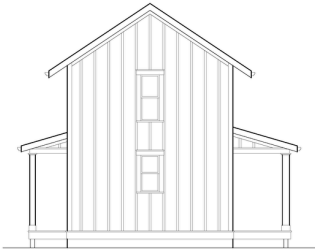
EAST ELEVATION
