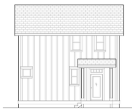
SOUTH ELEVATION
