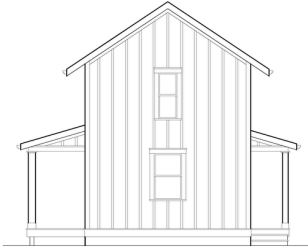
WEST ELEVATION
