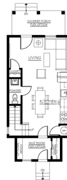
FIRST FLOOR PLAN (FLEX OPTIONS)
