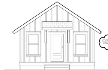
NORTH ELEVATION
