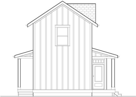
LEFT ELEVATION
