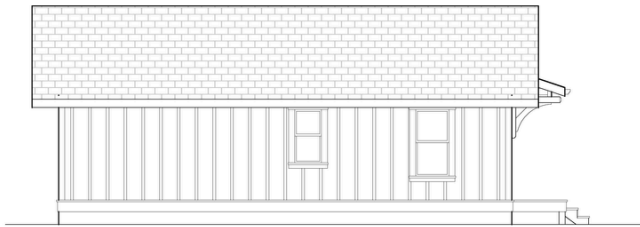
WEST ELEVATION
