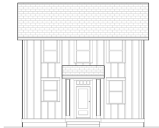
NORTH ELEVATION
