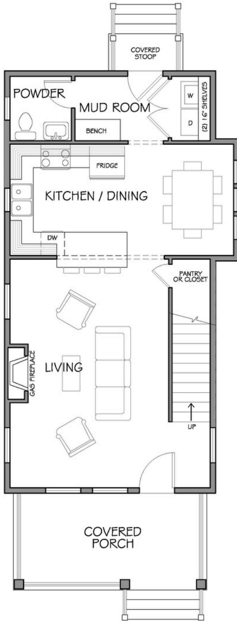
MAIN LEVEL
