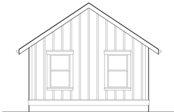
SOUTH ELEVATION
