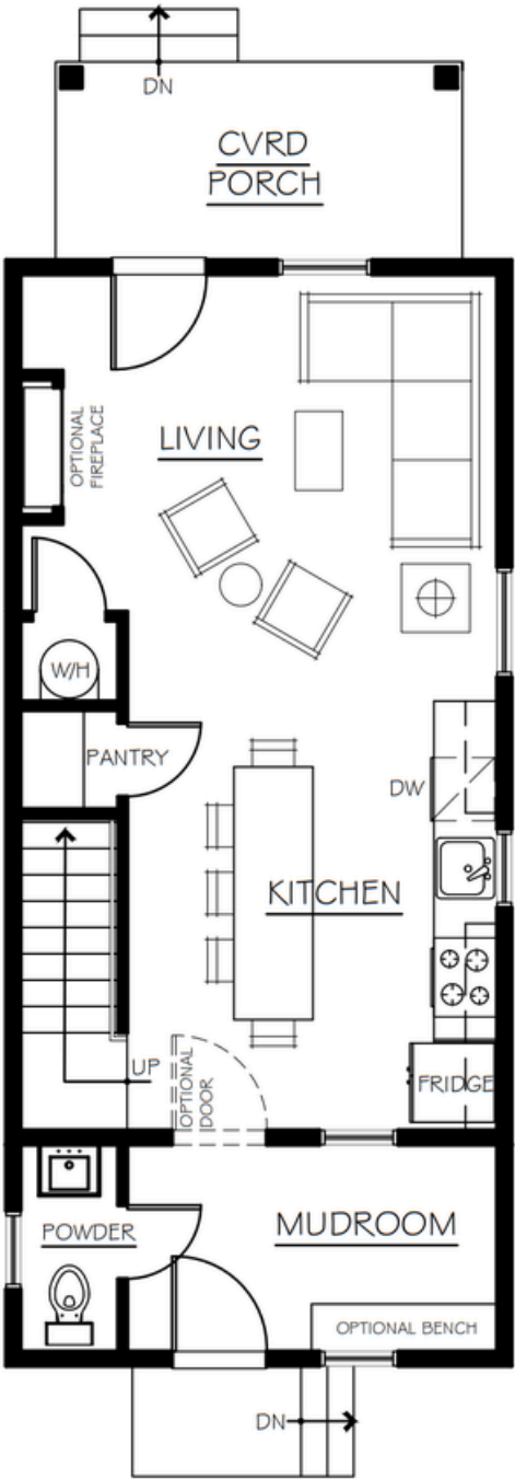
MAIN LEVEL
