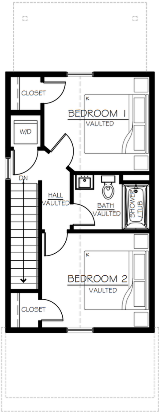
UPPER LEVEL
