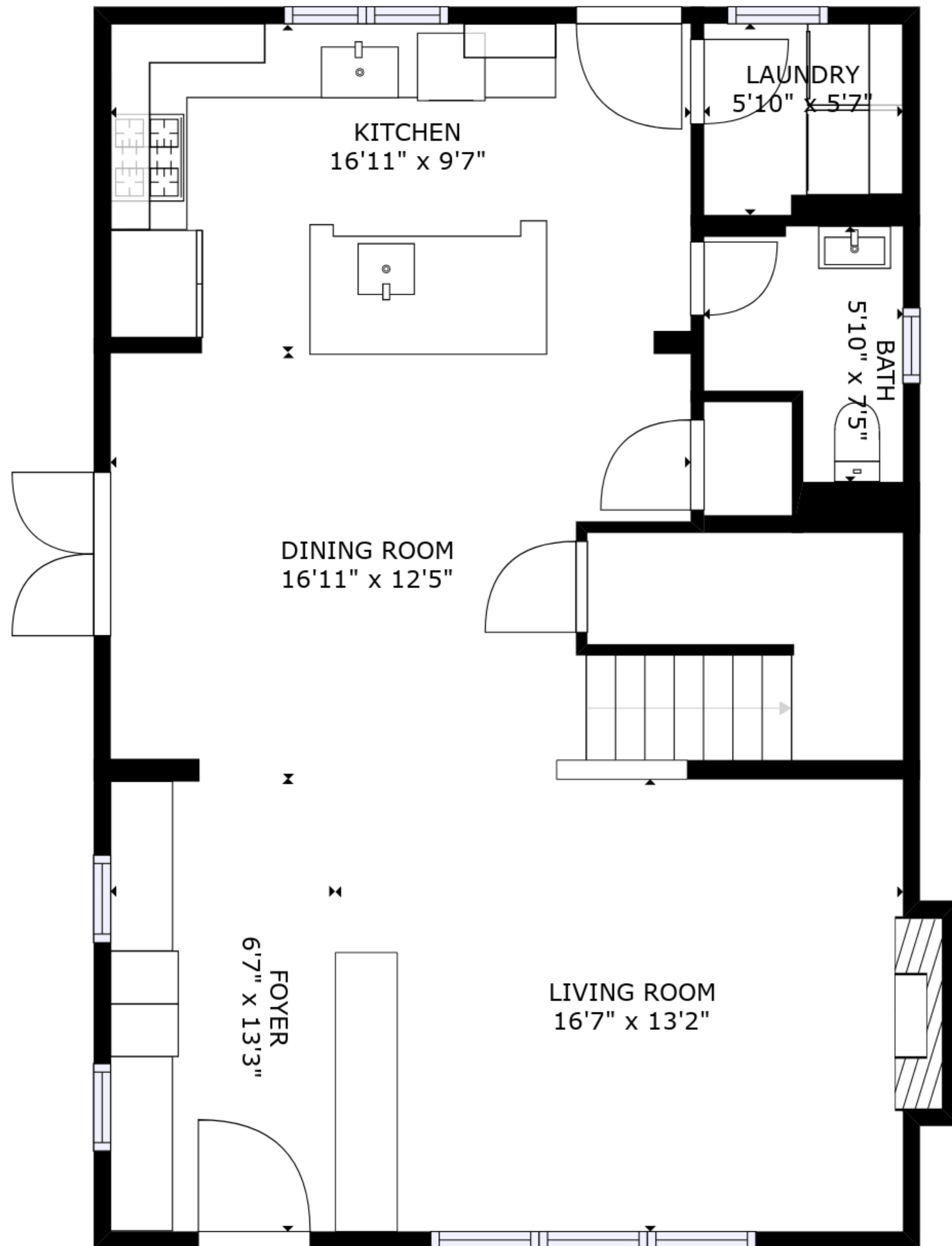
FLOOR 1
