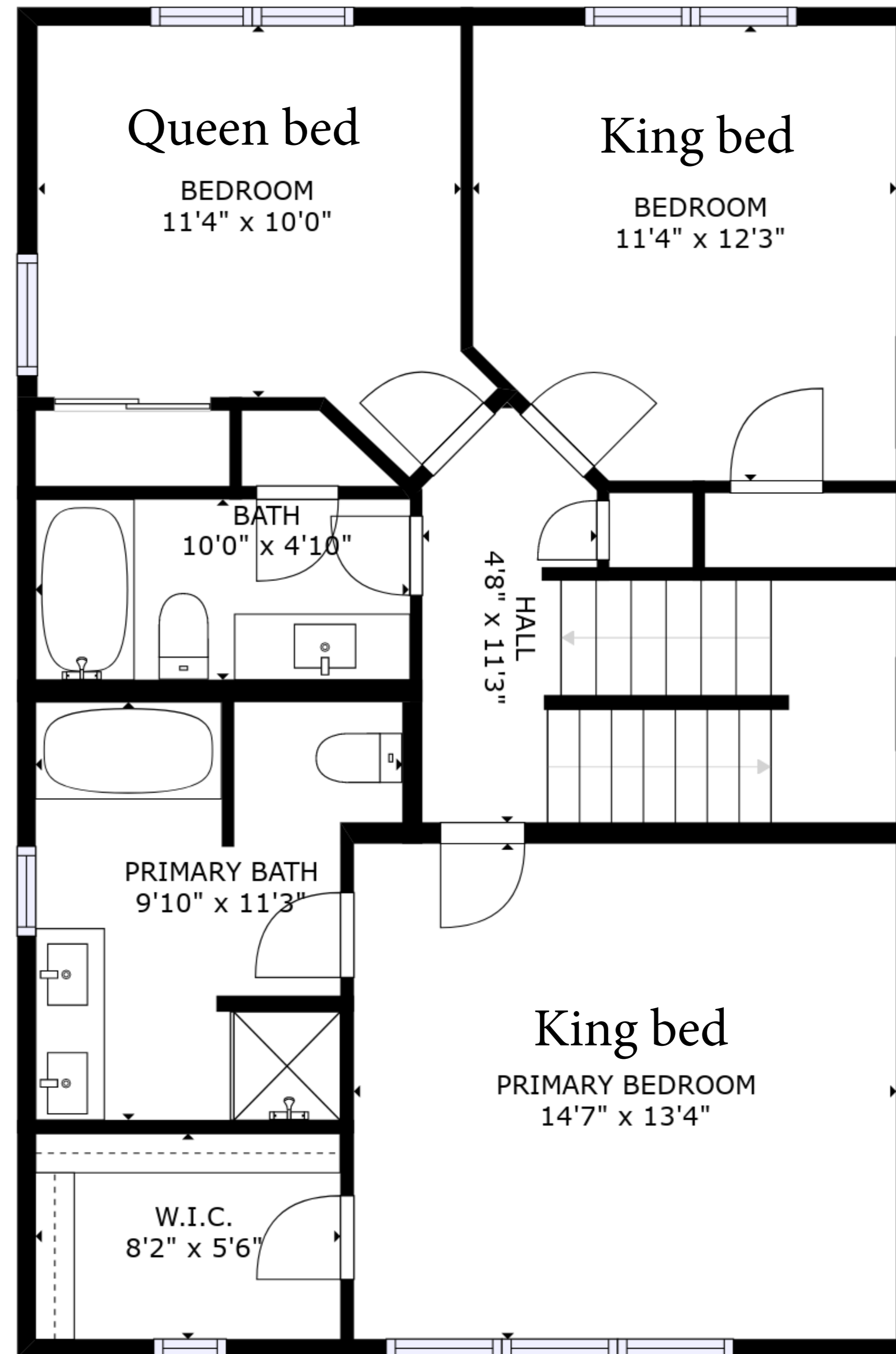
FLOOR 2
