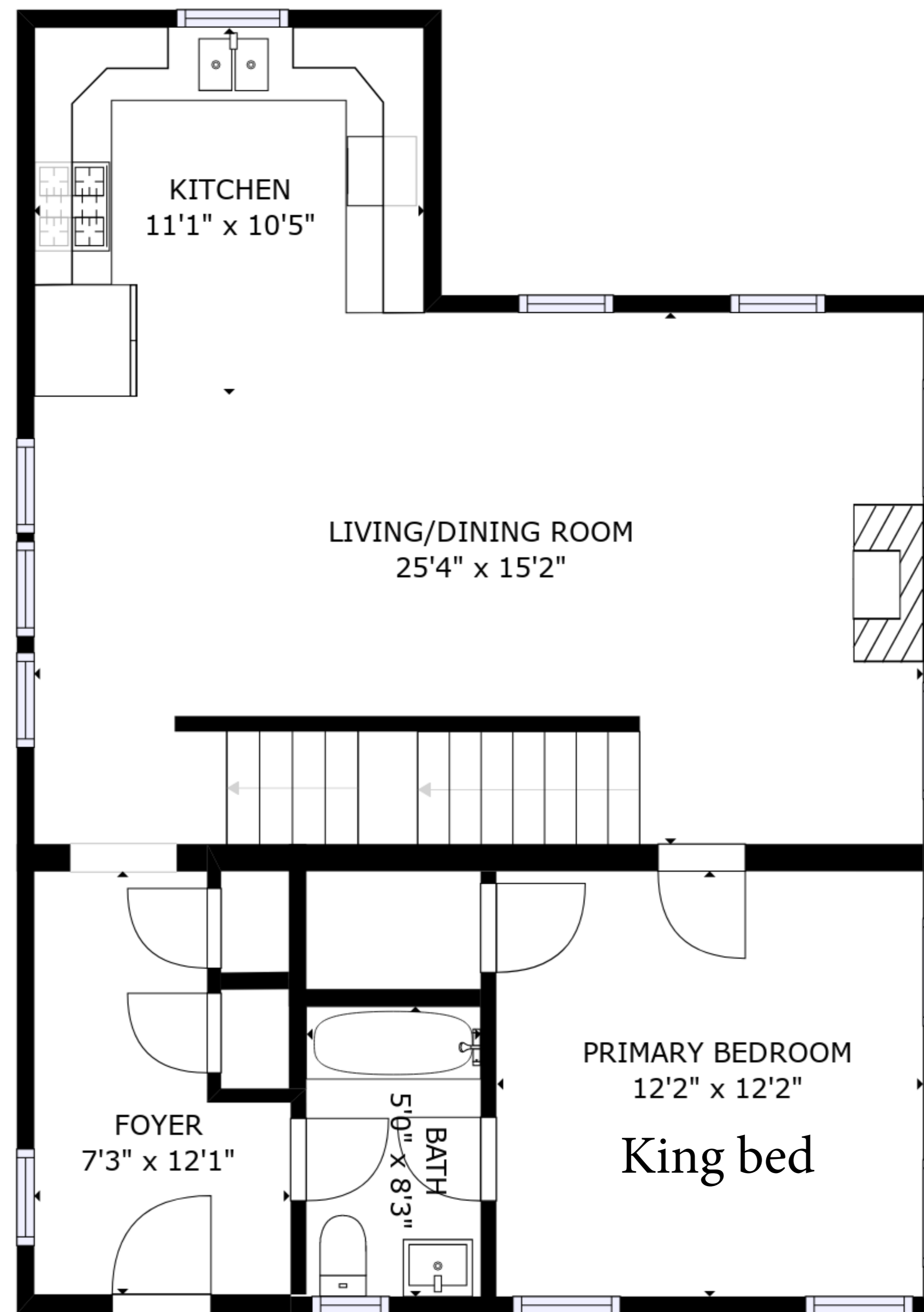
FLOOR 2
