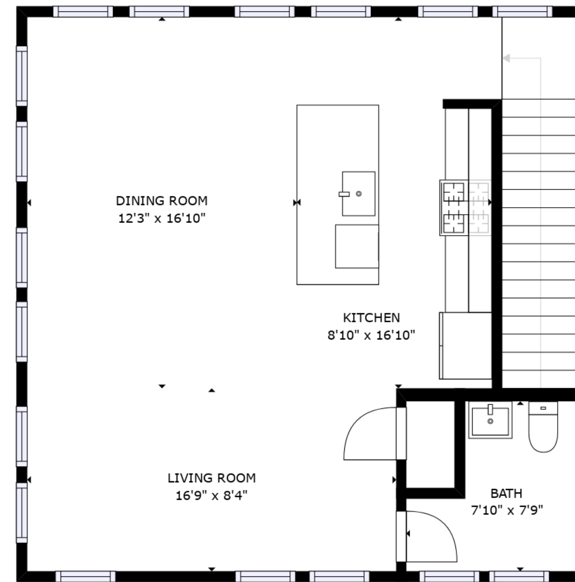
FLOOR 3
