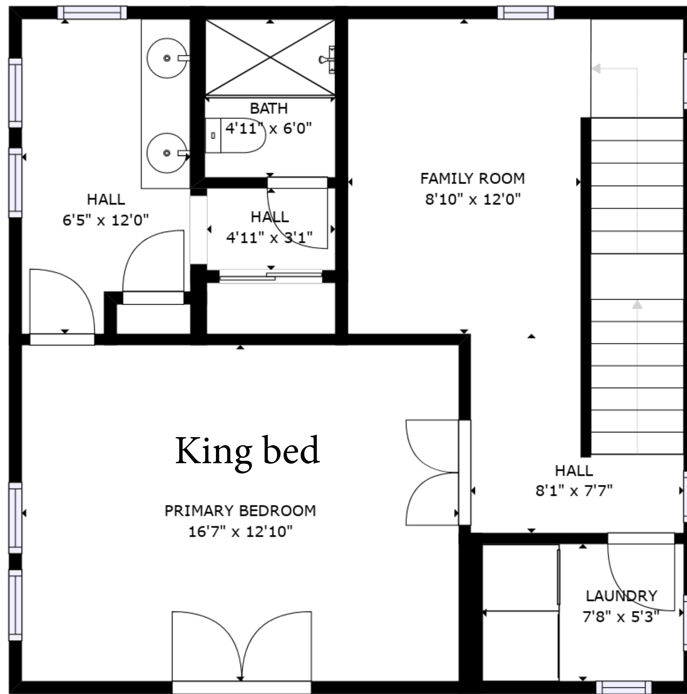
FLOOR 2
