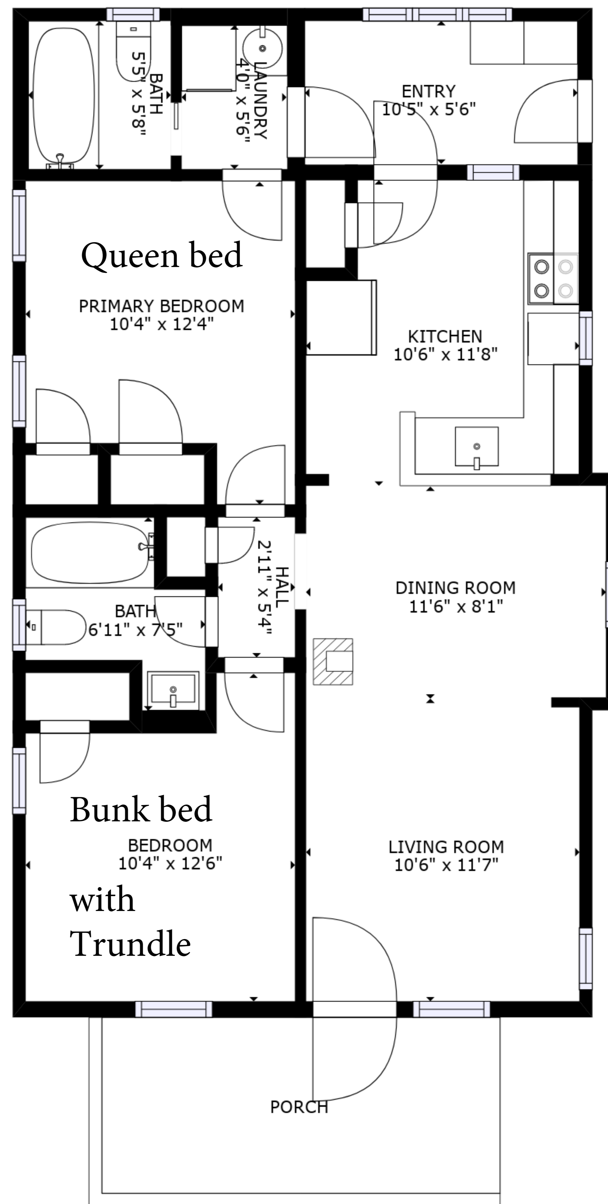
FLOOR 1
