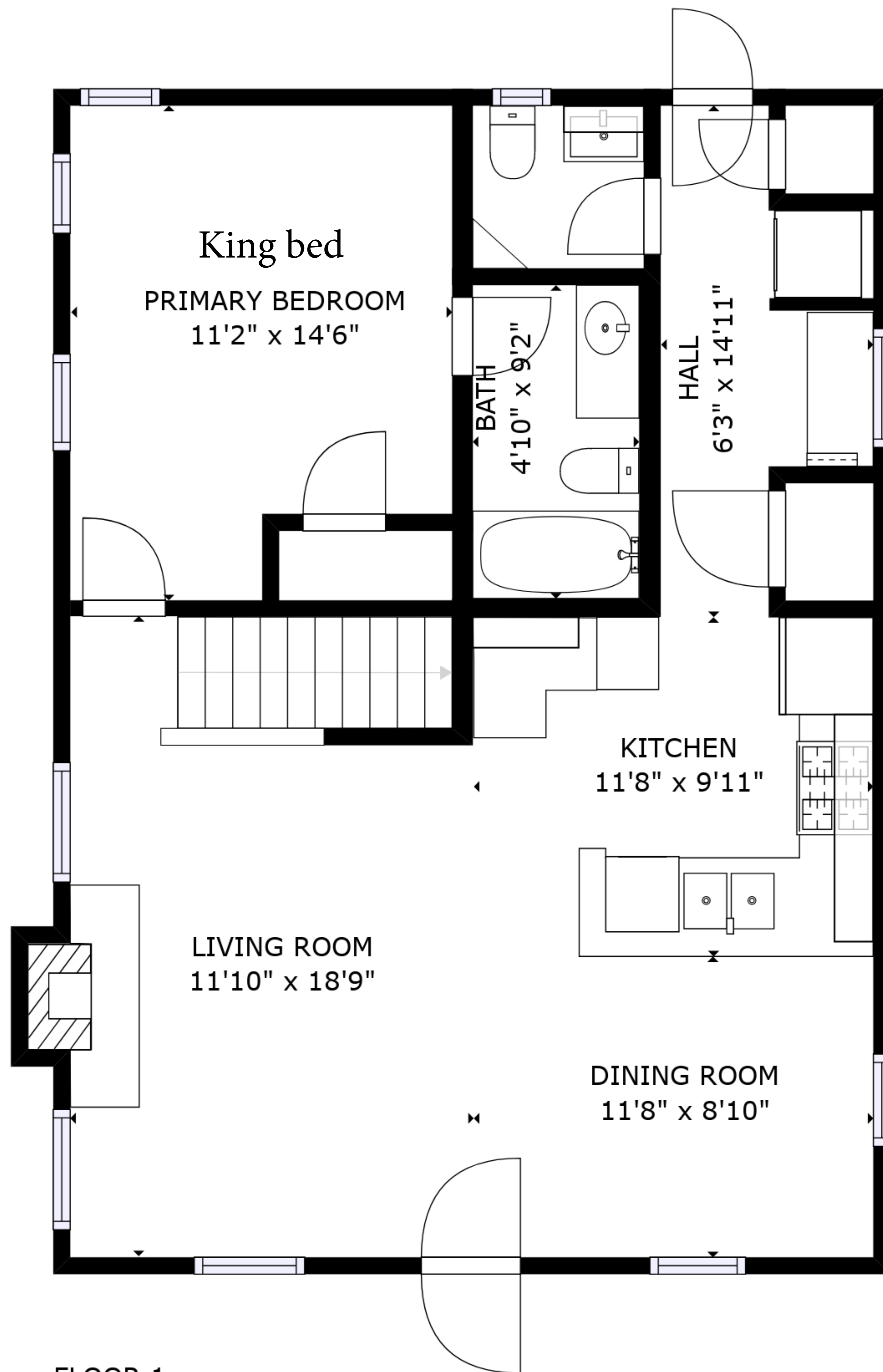
FLOOR 1
