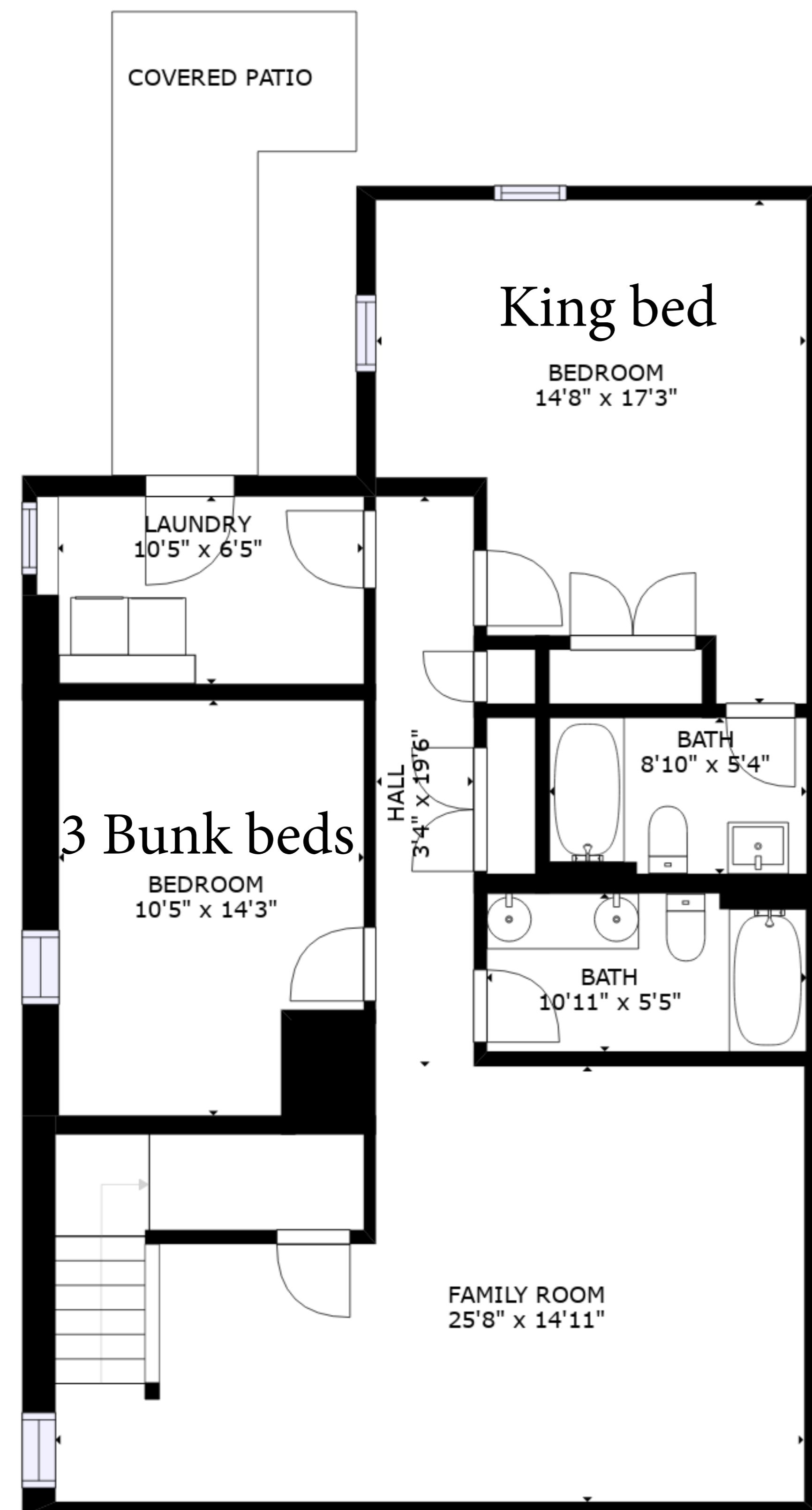
FLOOR 1
