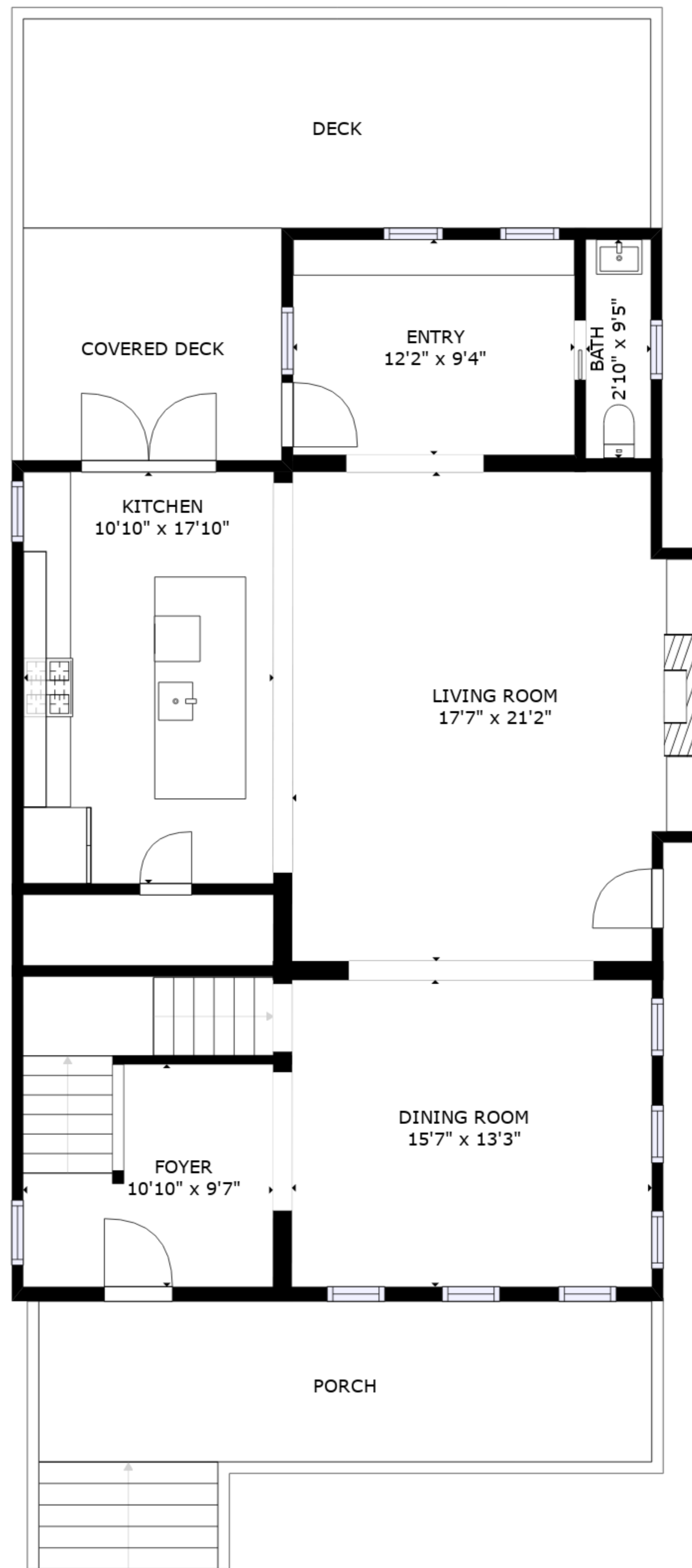
FLOOR 2
