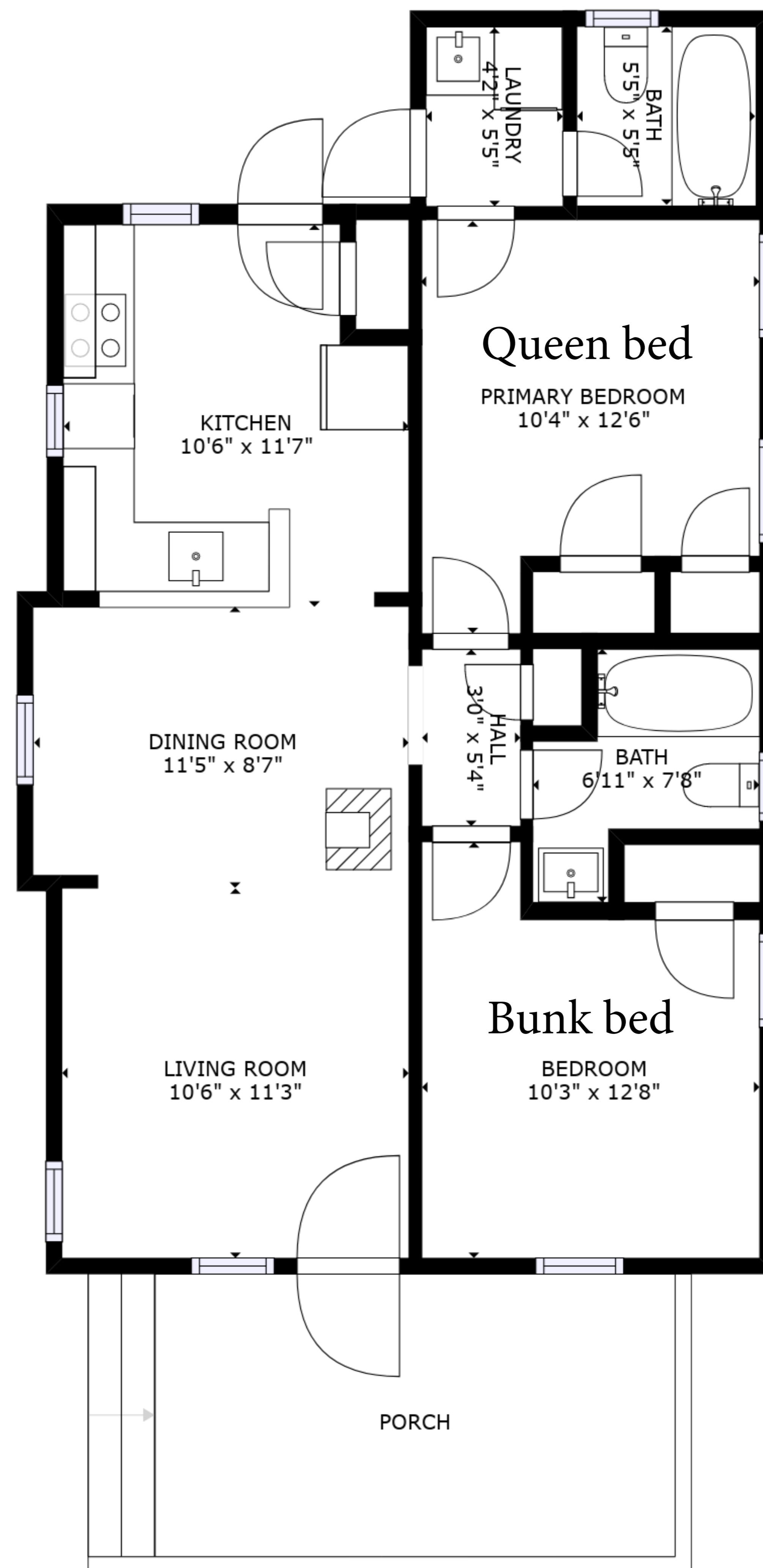
FLOOR 1
