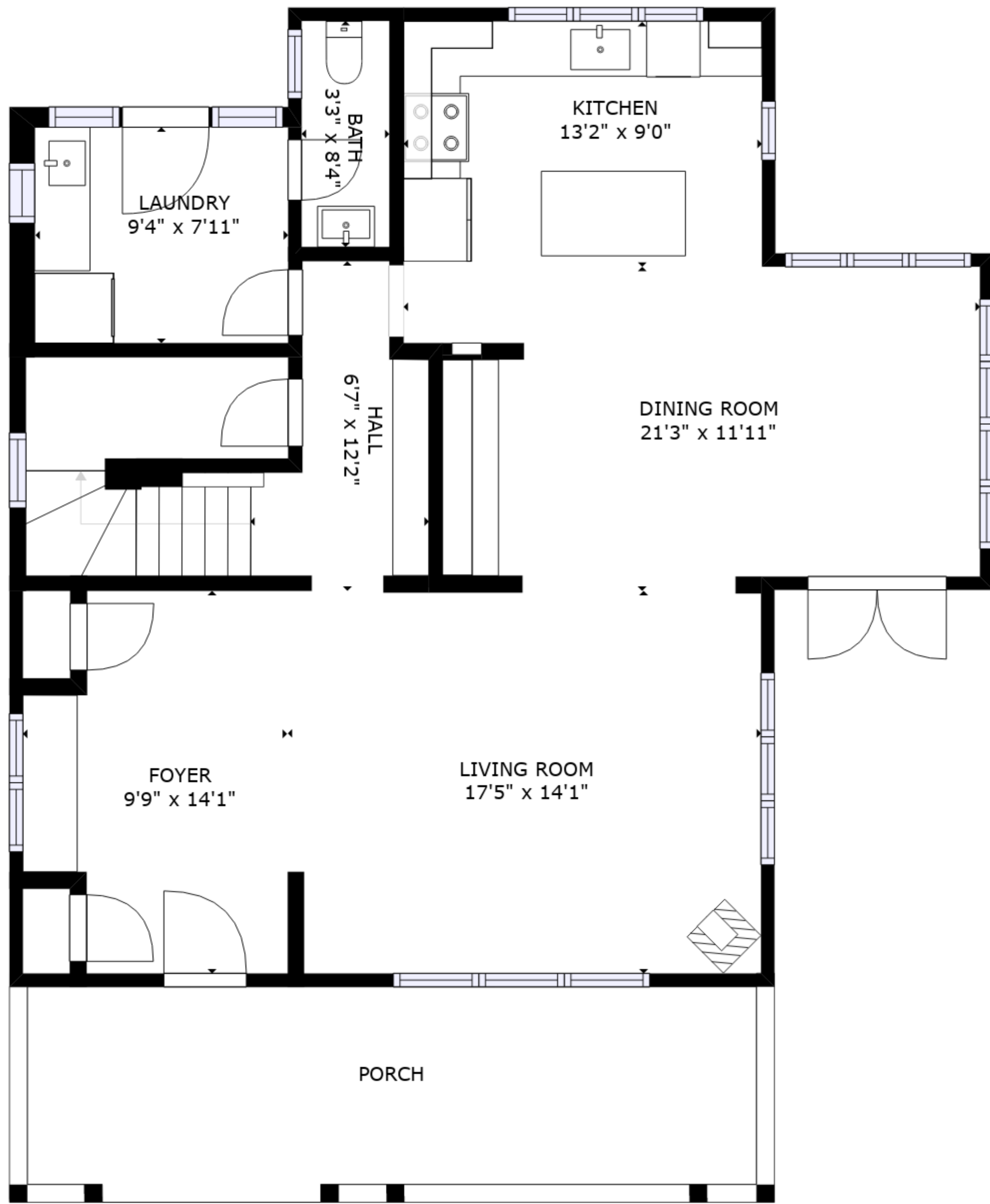
FLOOR 1
