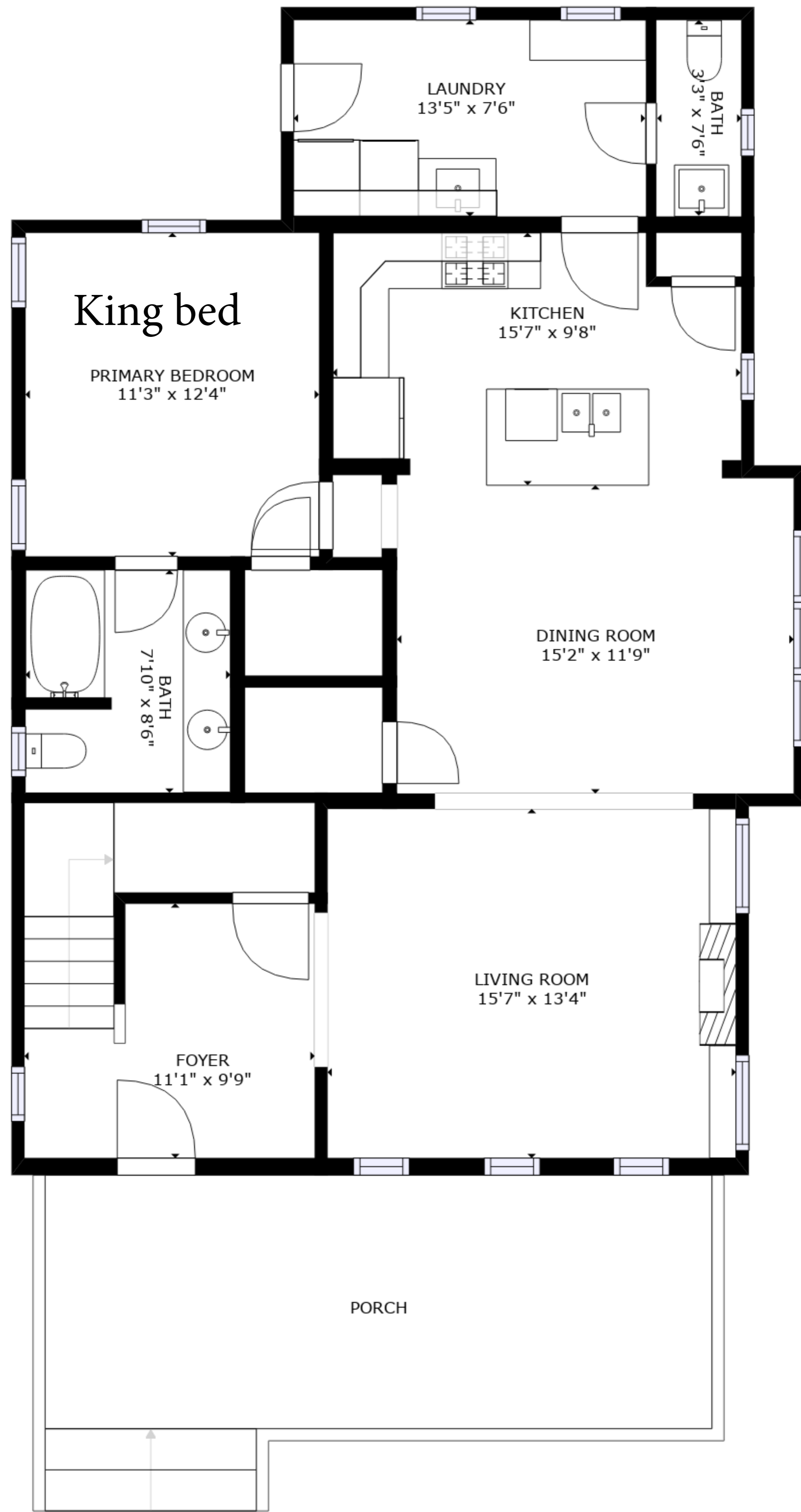
FLOOR 1
