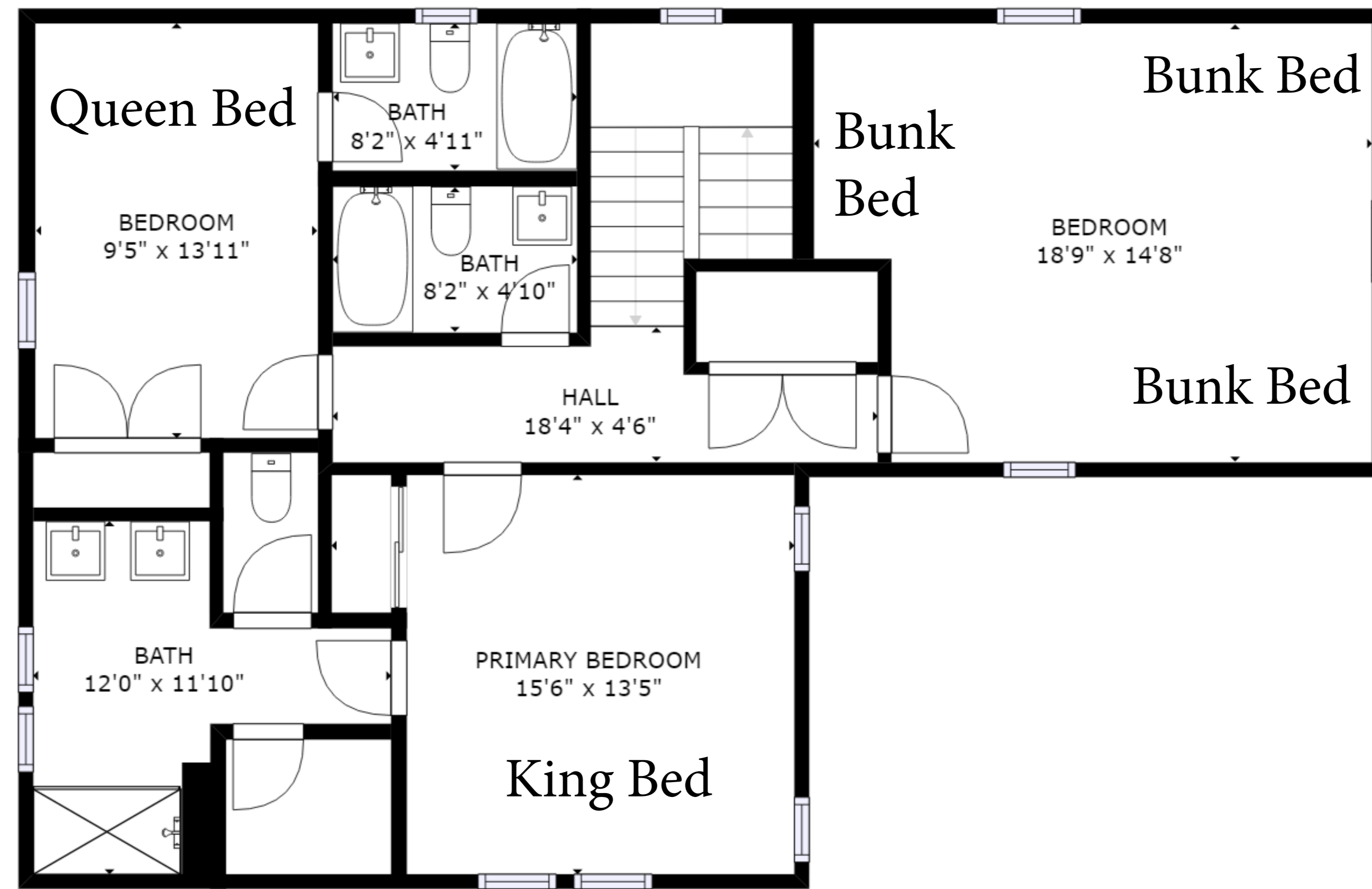
FLOOR 2
