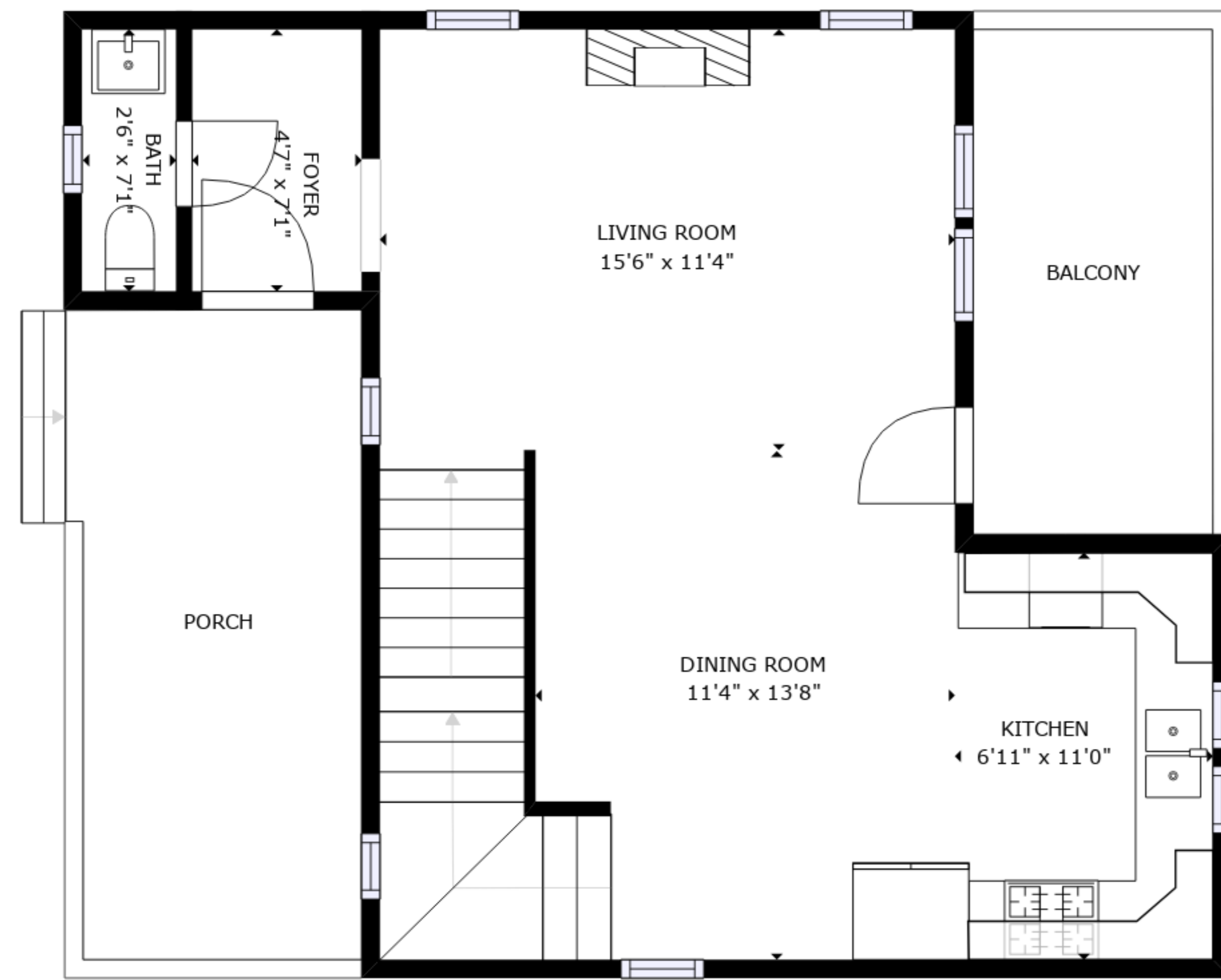
FLOOR 2
