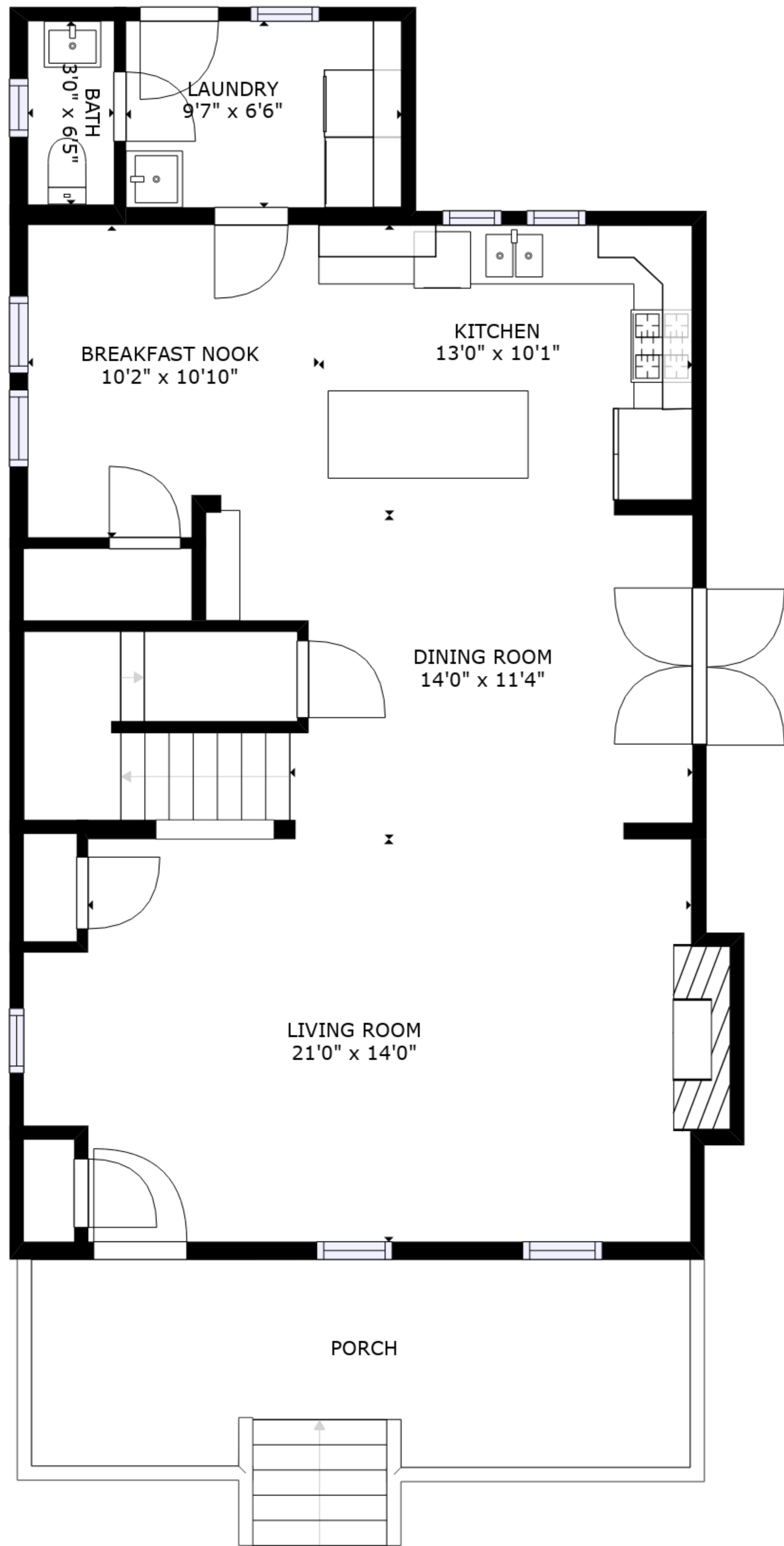
FLOOR 1
