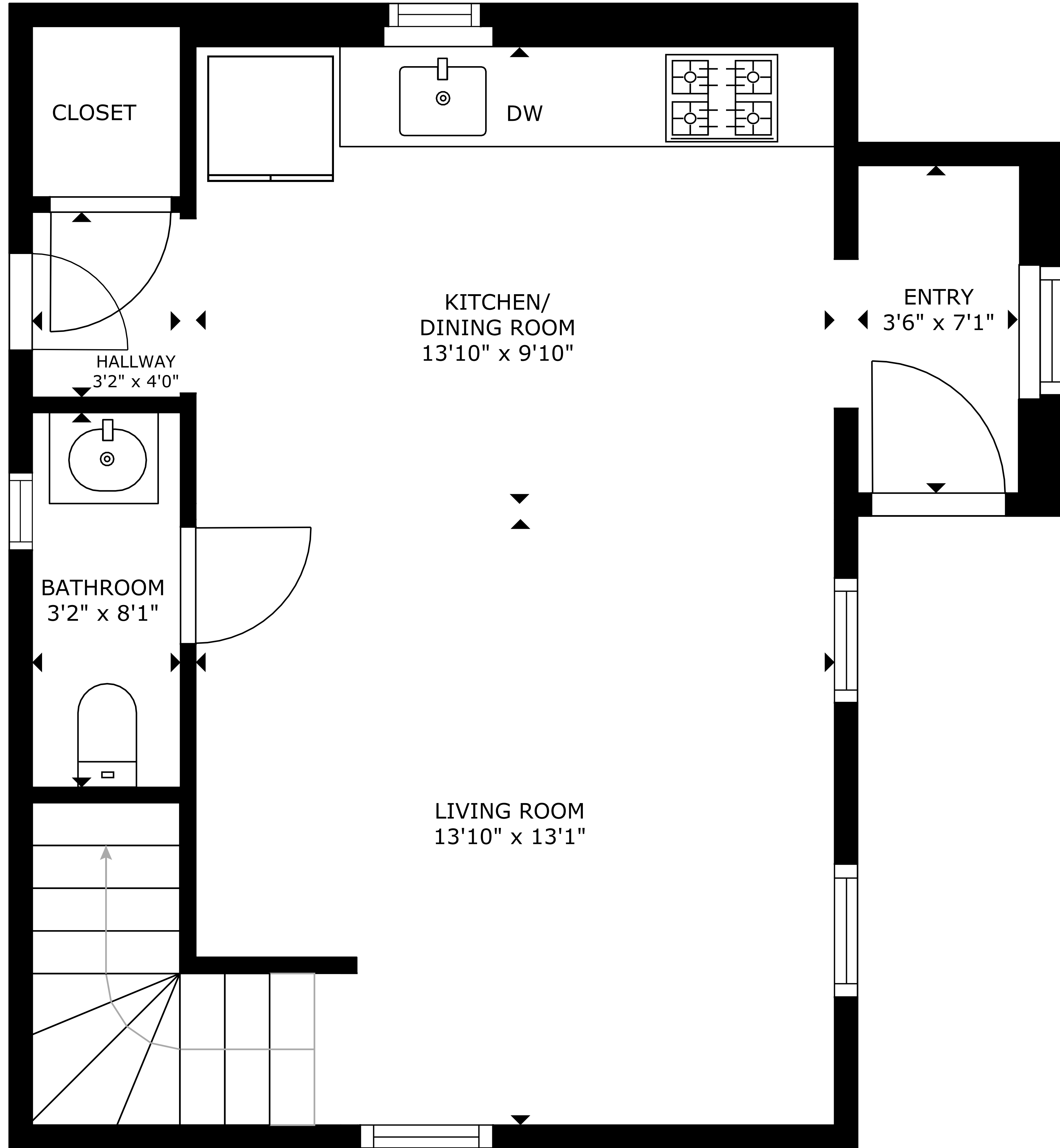
FLOOR 1
